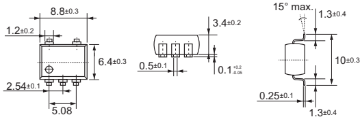
Surface-mounting Terminals
