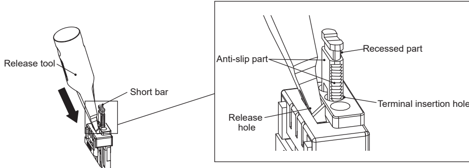
Fig 1: Removing the short bar from the terminal block
