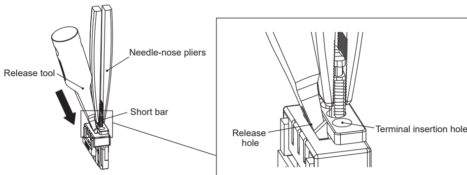
Fig 2: Removing the short bar from the terminal block with needle-nose pliers.
