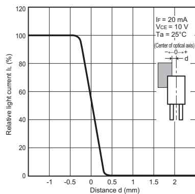
Fig 10. Sensing Position Characteristics (Typical) EE-SJ3-C
