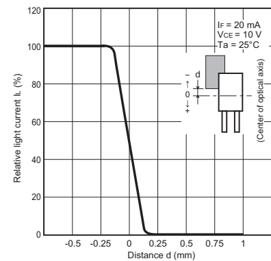
Fig 9. Sensing Position Characteristics (Typical) EE-SJ3-G
