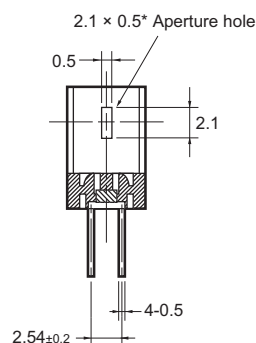
Cross section view A-A
