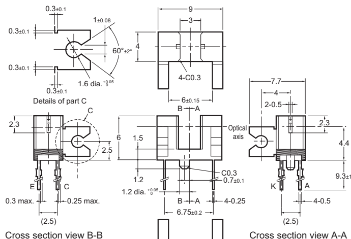
Cross section view B-B
