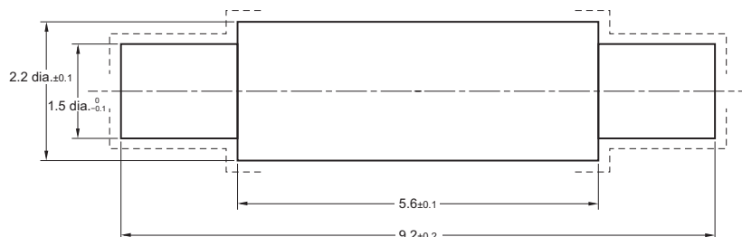
Reference Actuator Design Drawing
