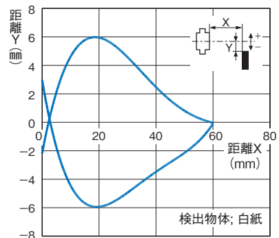
形B5W-LB2□
