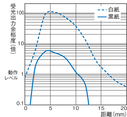
形B5W-LB1□
