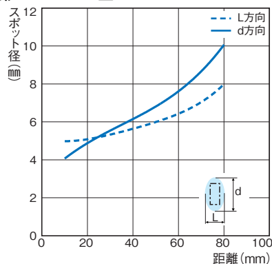
形B5W-LB2□
