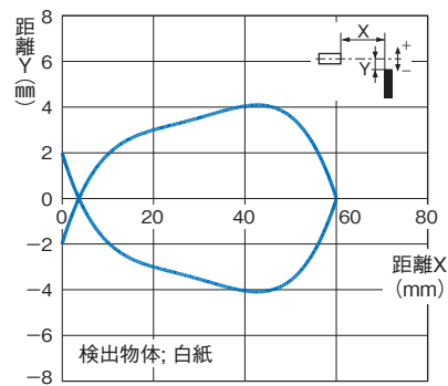
形B5W-LB2□
