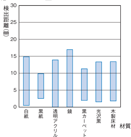
形B5W-LB1□
