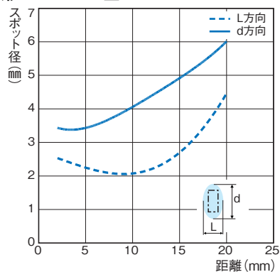
形B5W-LB1□
