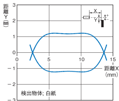
形B5W-LB1□
