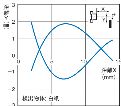
形B5W-LB1□
