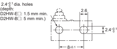
Mounting Hole Dimensions (Reference)
