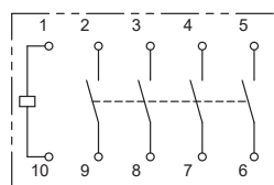
Terminal Arrangement/ Internal Connections (BOTTOM VIEW)
