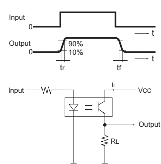
Fig 12. Response Time Measurement Circuit
