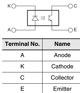
Internal circuit
