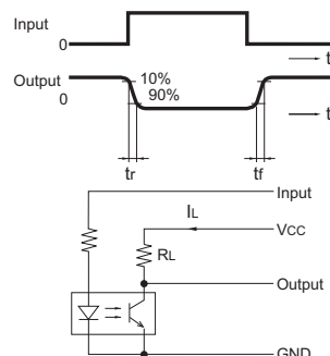
Fig 10. Response Time Measurement Circuit
