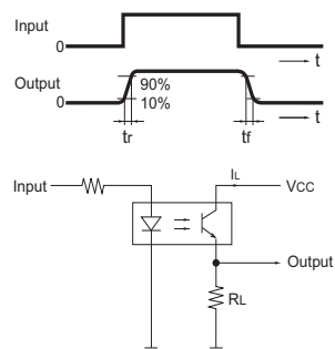
Fig 10. Response Time Measurement Circuit
