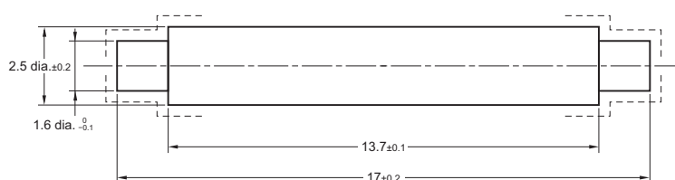
Reference Actuator Design Drawing
