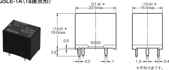
形G5LE-1 (1c接点形) 形G5LE-1A (1a接点形)
