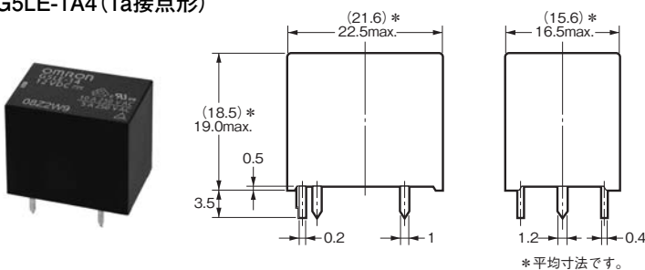
形G5LE-14 (1c接点形) 形G5LE-1A4 (1a接点形)
