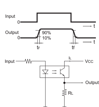
Fig 12. Response Time Measurement Circuit
