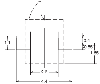
PCB pad dimensions (reference) (TOP VIEW)
