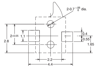
PCB mounting hole and pad dimensions (reference) (TOP VIEW)
