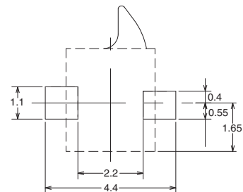
PCB pad dimensions (reference) (TOP VIEW)
