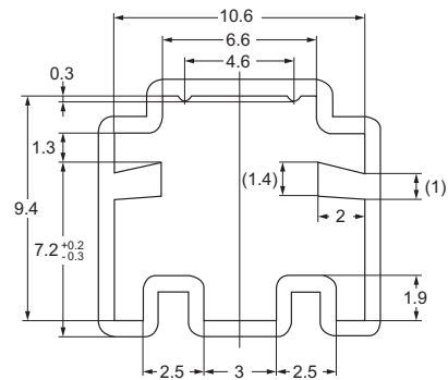
Plastic sleeve size
